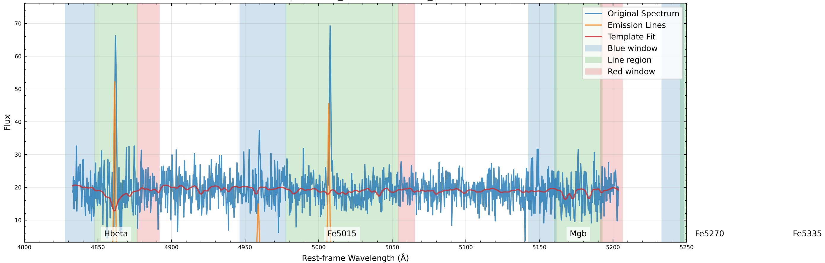
Original Data Comparison (v_star=30.2 km/s, v_gas=49.3 km/s)
