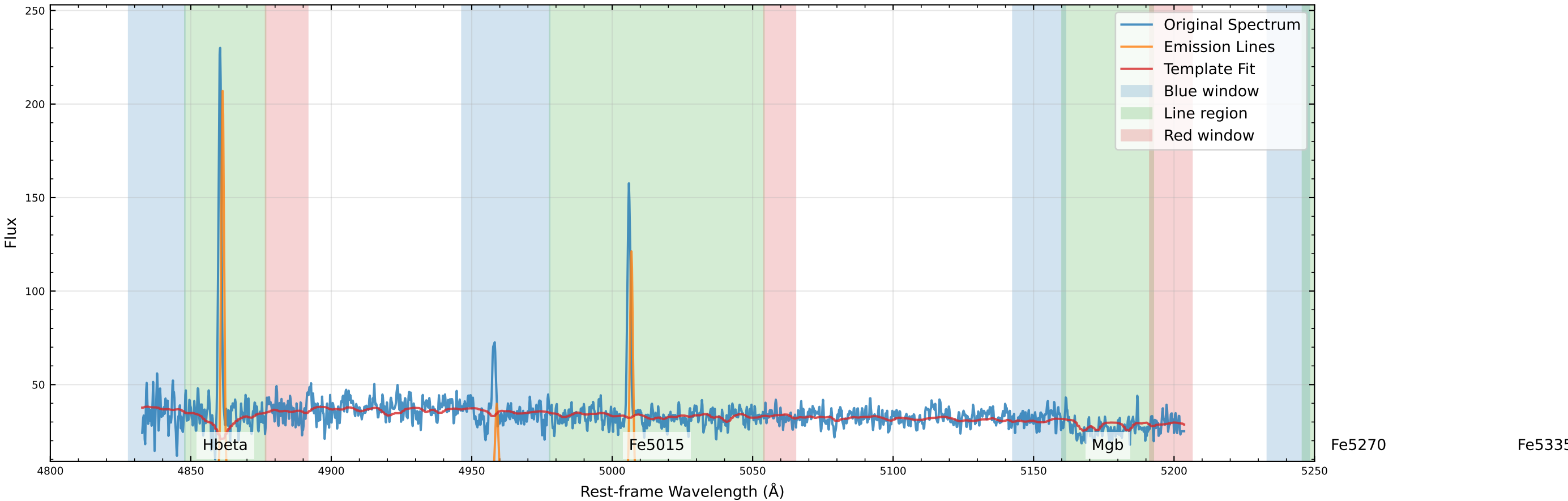
Original Data Comparison (v_star=-128.5 km/s, v_gas=-56.5 km/s)
