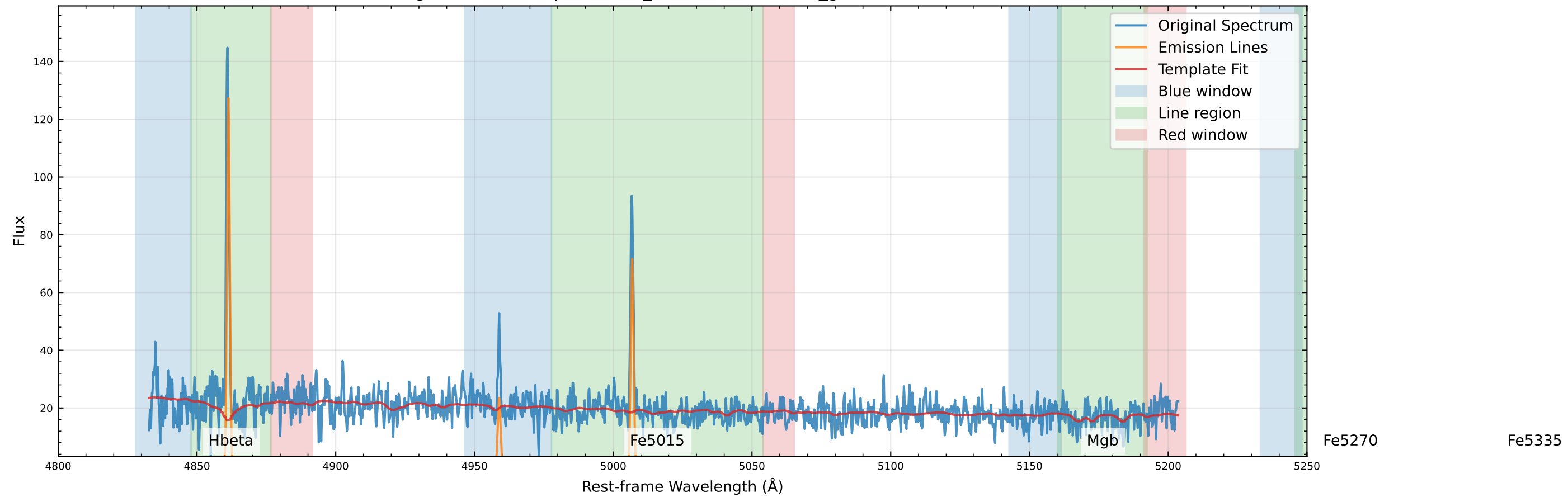
Original Data Comparison (v_star=-38.0 km/s, v_gas=-16.3 km/s)
