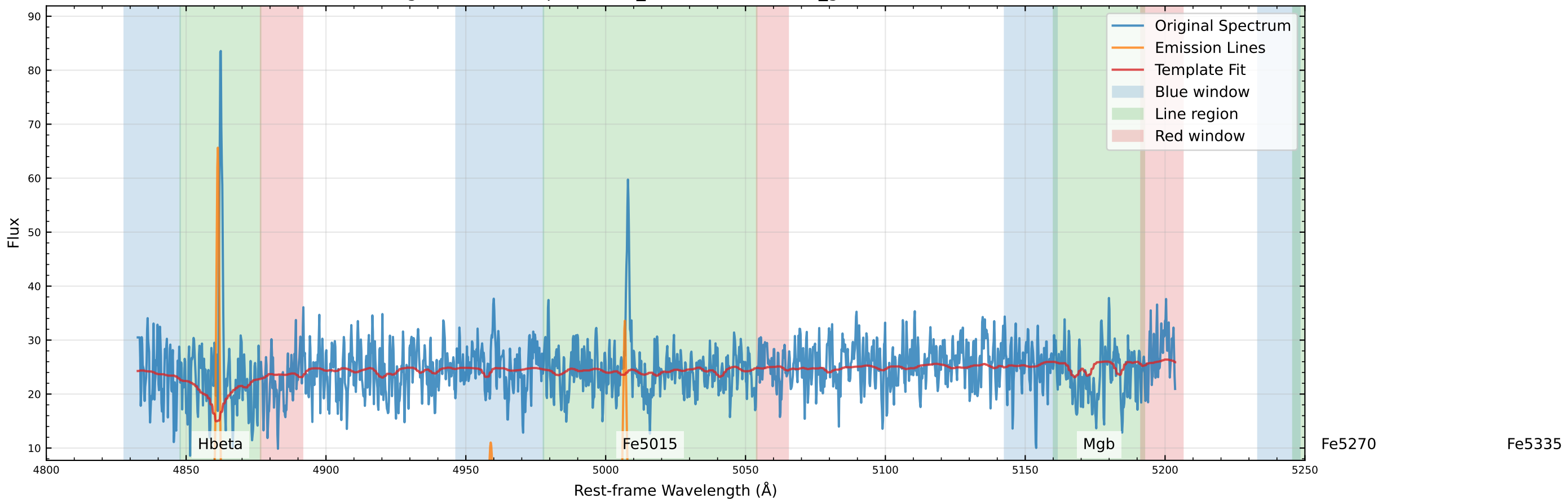
Original Data Comparison (v_star=104.3 km/s, v_gas=66.8 km/s)
