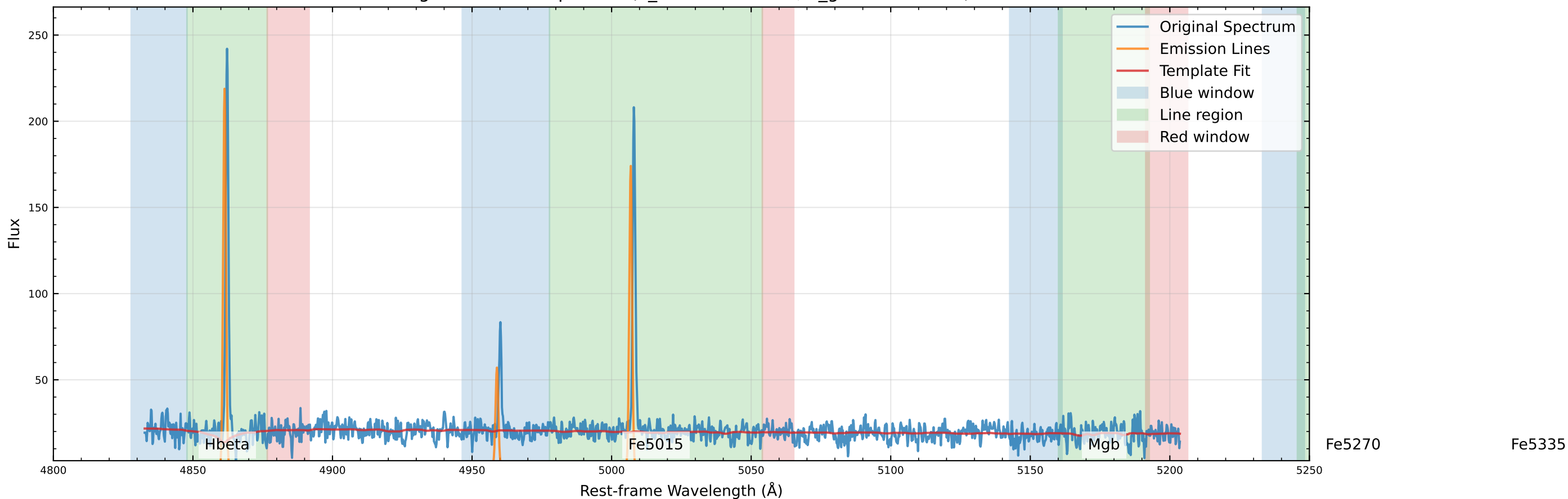
Original Data Comparison (v_star=83.3 km/s, v_gas=61.7 km/s)
