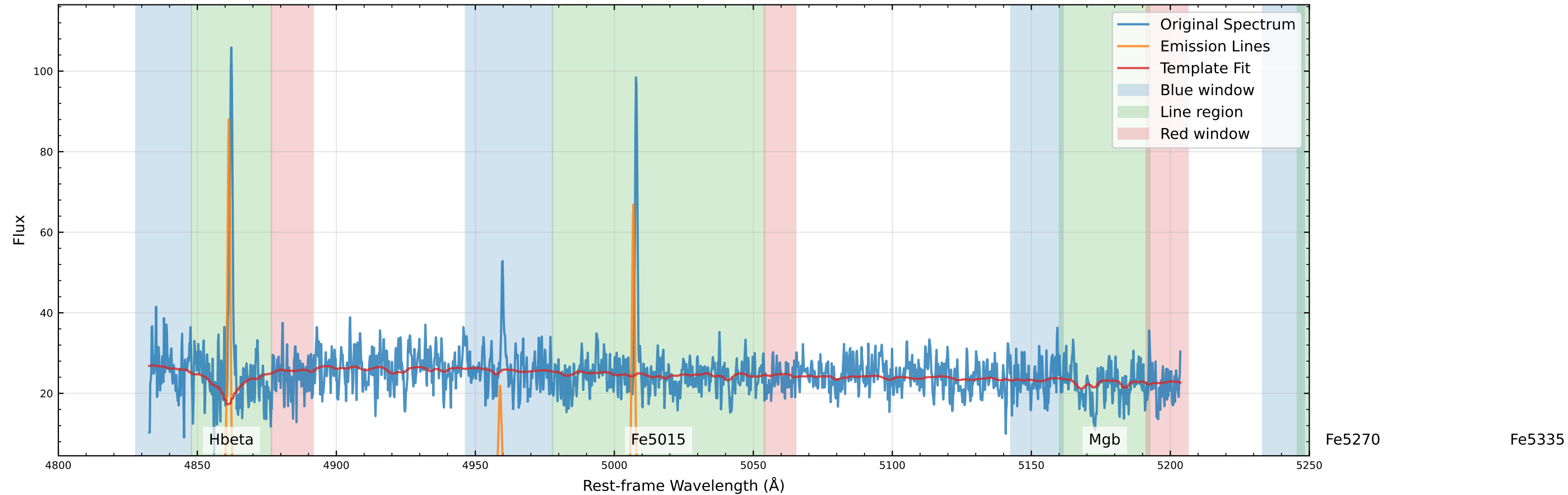
Original Data Comparison (v_star=22.1 km/s, v_gas=56.2 km/s)
