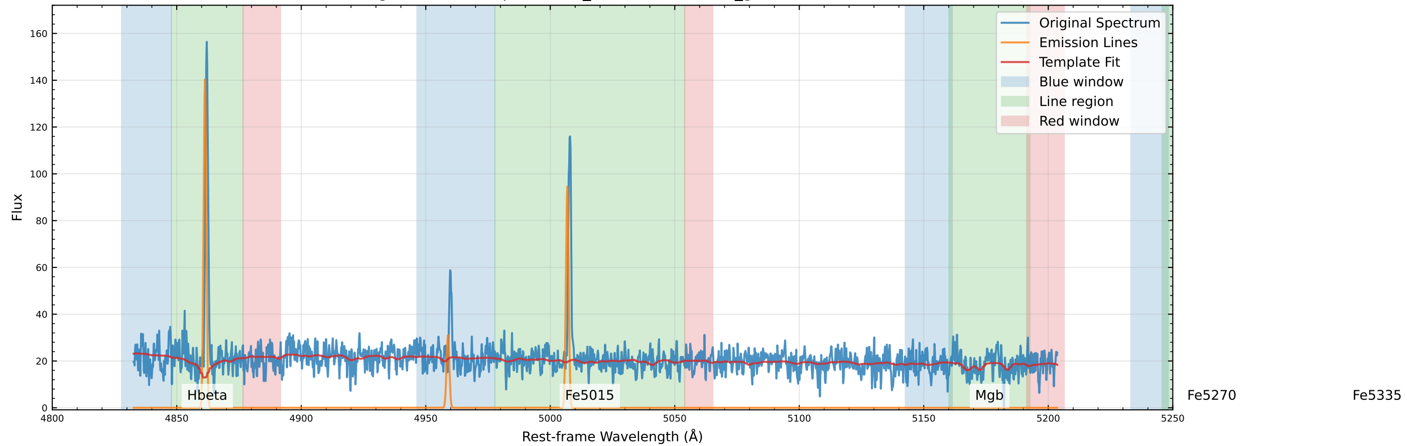
Original Data Comparison (v_star=22.6 km/s, v_gas=48.6 km/s)
