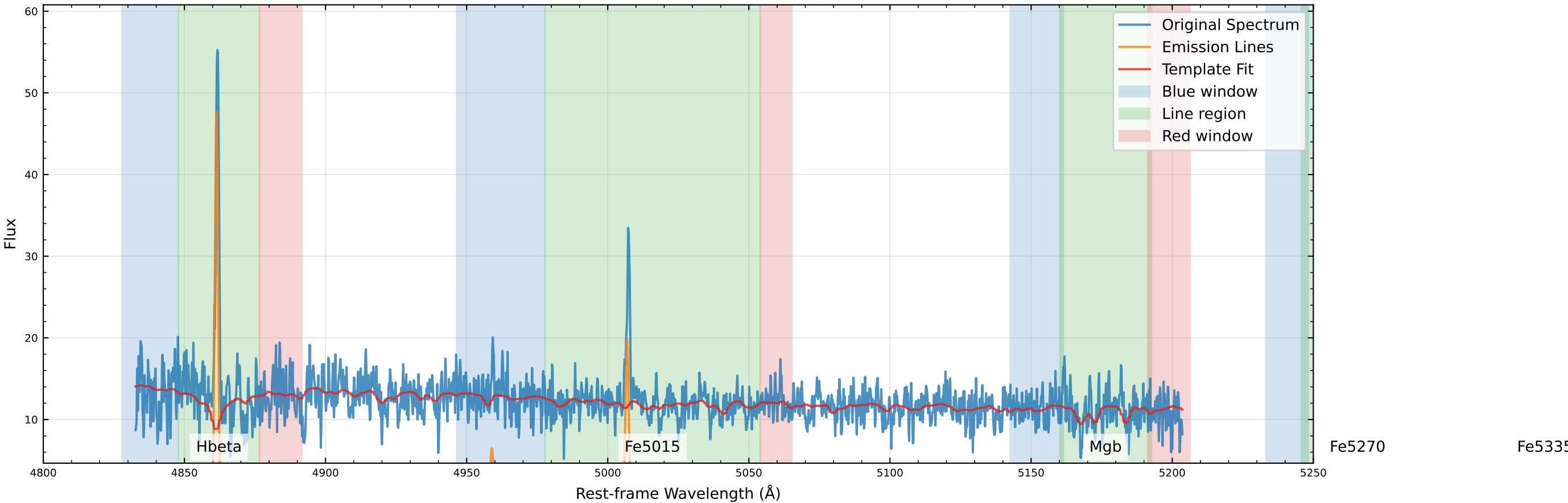
Original Data Comparison (v_star=21.8 km/s, v_gas=22.7 km/s)
