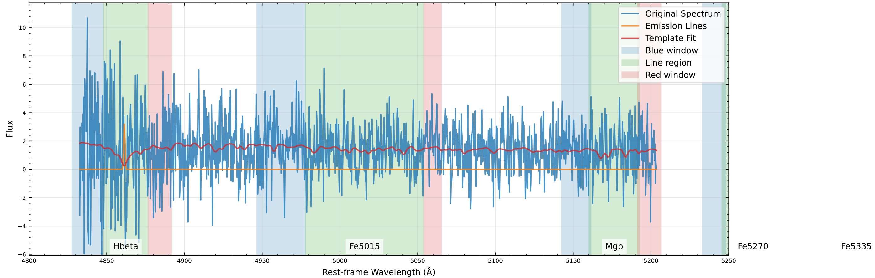
Original Data Comparison (v_star=-27.6 km/s, v_gas=-46.3 km/s)
