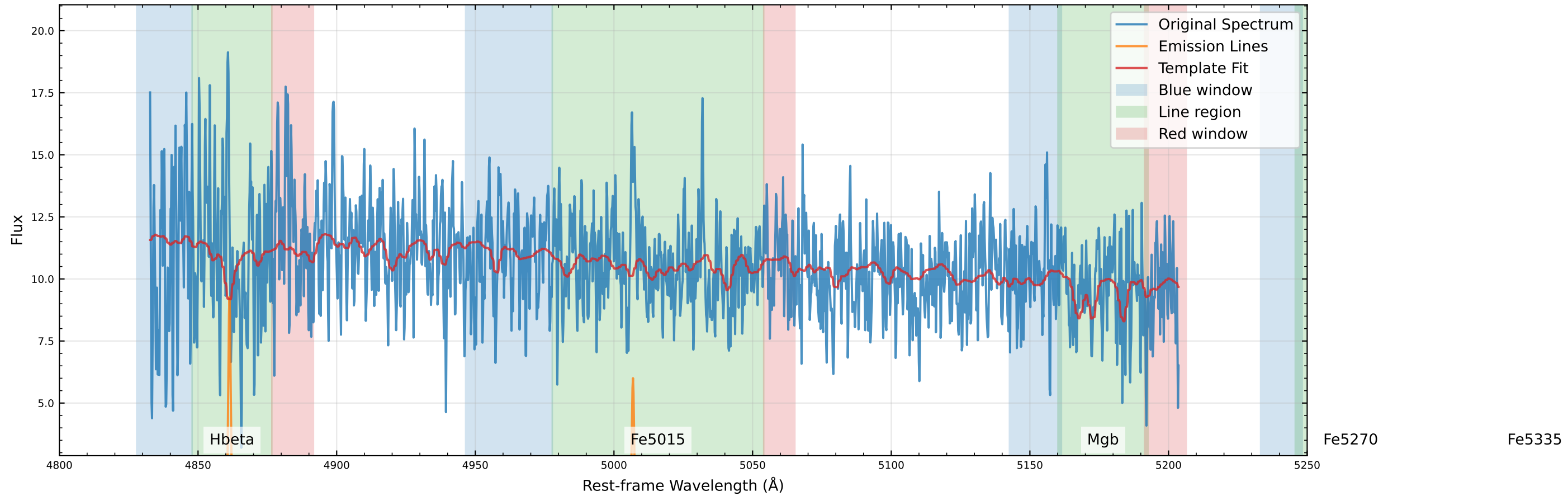
Original Data Comparison (v_star=-43.7 km/s, v_gas=-29.4 km/s)
