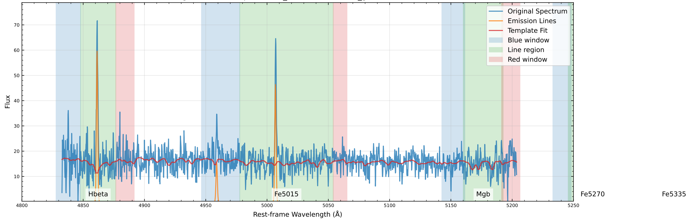
Original Data Comparison (v_star=13.4 km/s, v_gas=10.2 km/s)
