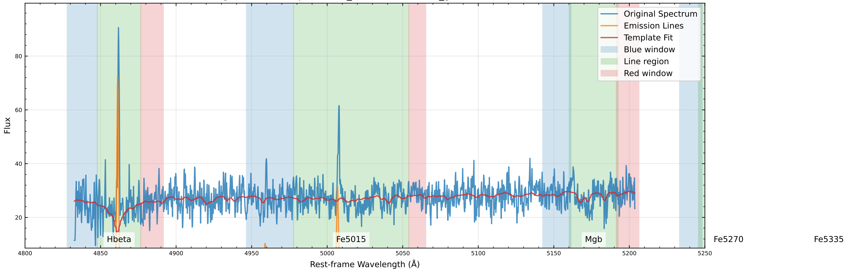
Original Data Comparison (v_star=57.3 km/s, v_gas=36.7 km/s)
