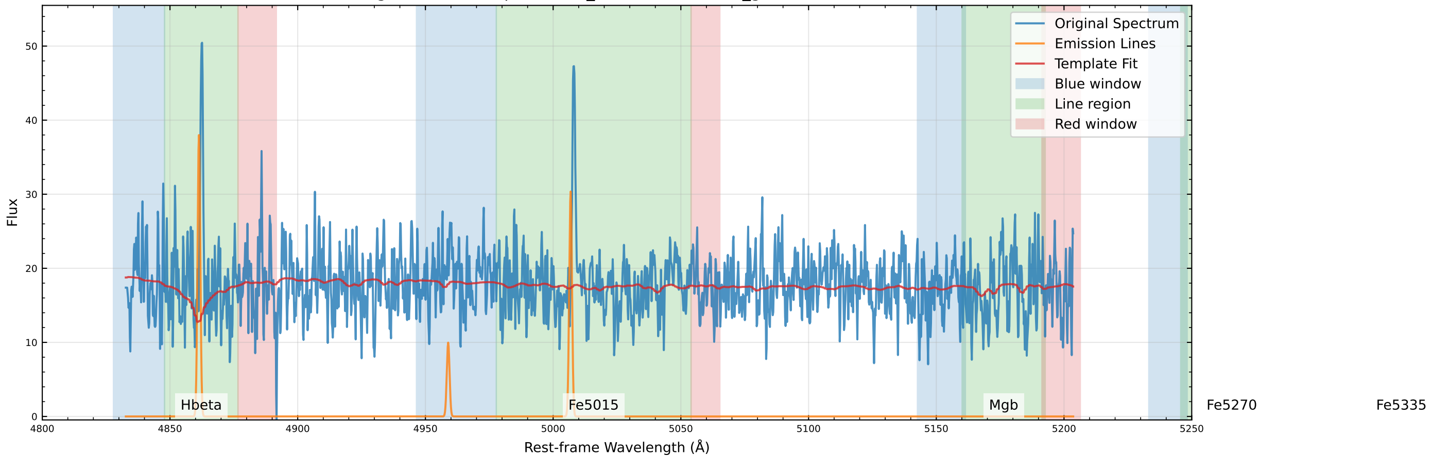
Original Data Comparison (v_star=71.1 km/s, v_gas=69.9 km/s)
