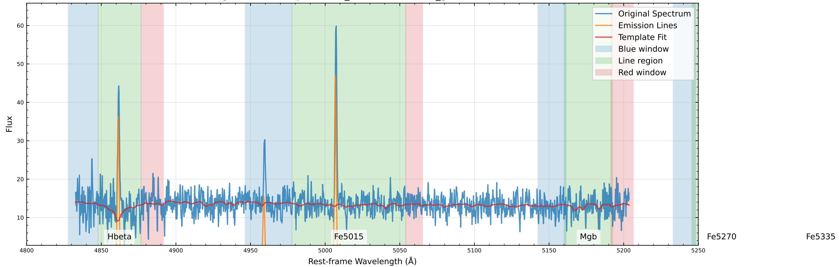
Original Data Comparison (v_star=30.6 km/s, v_gas=24.0 km/s)
