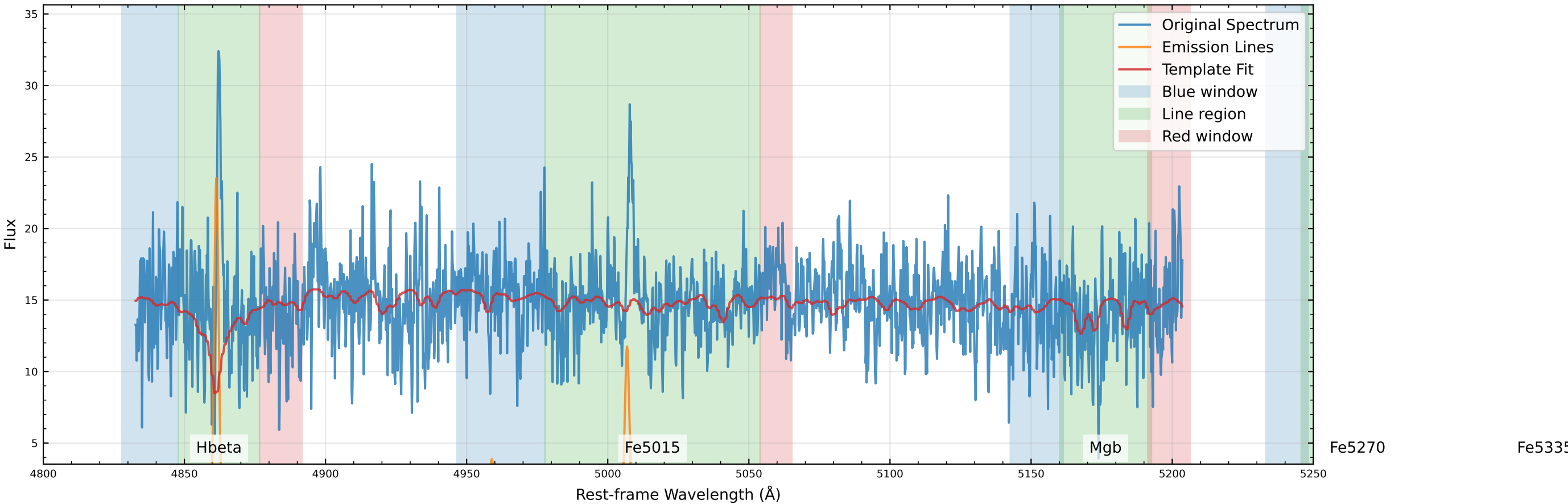
Original Data Comparison (v_star=111.7 km/s, v_gas=65.4 km/s)
