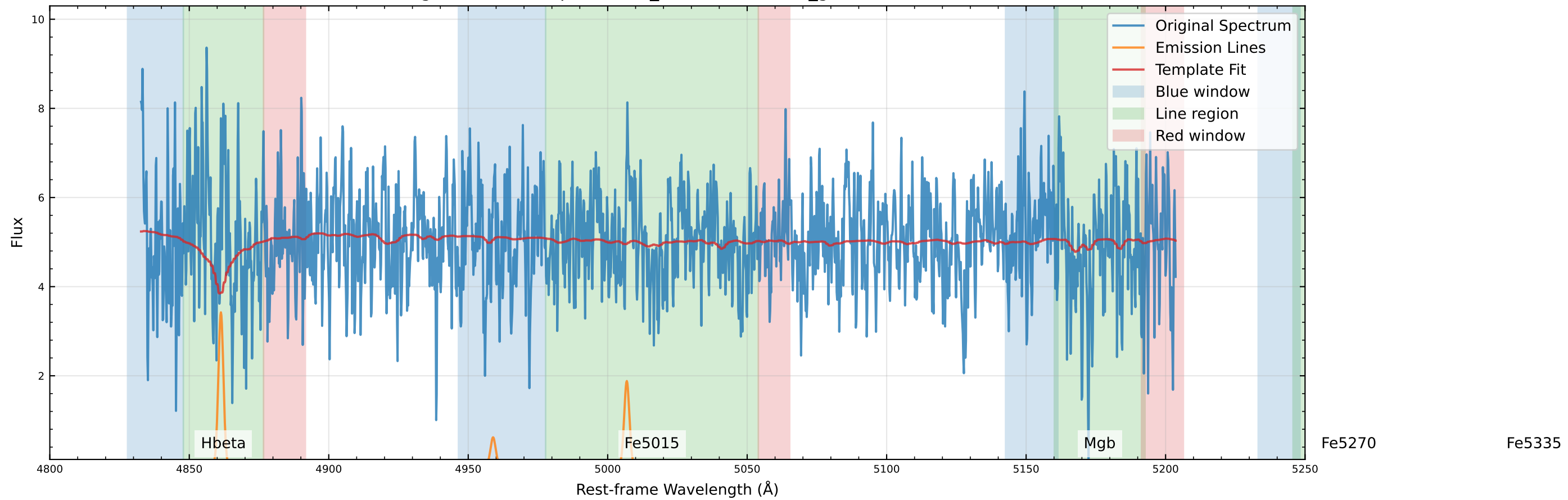
Original Data Comparison (v_star=6.6 km/s, v_gas=53.7 km/s)
