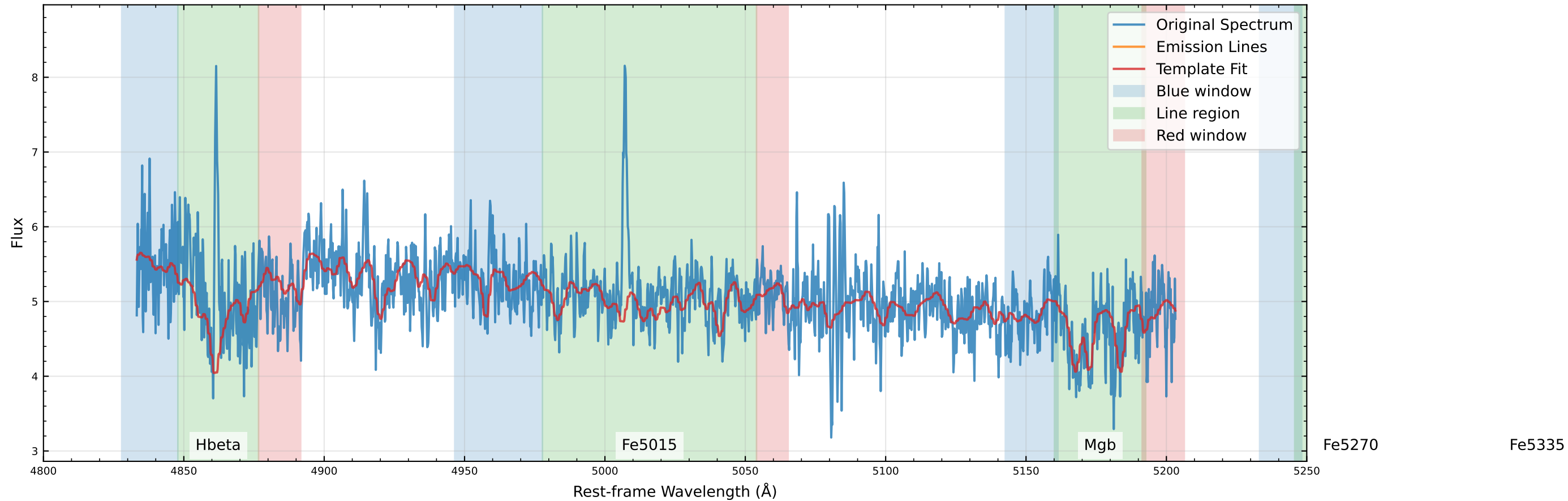
Original Data Comparison (v_star=-39.1 km/s, v_gas=20.6 km/s)
