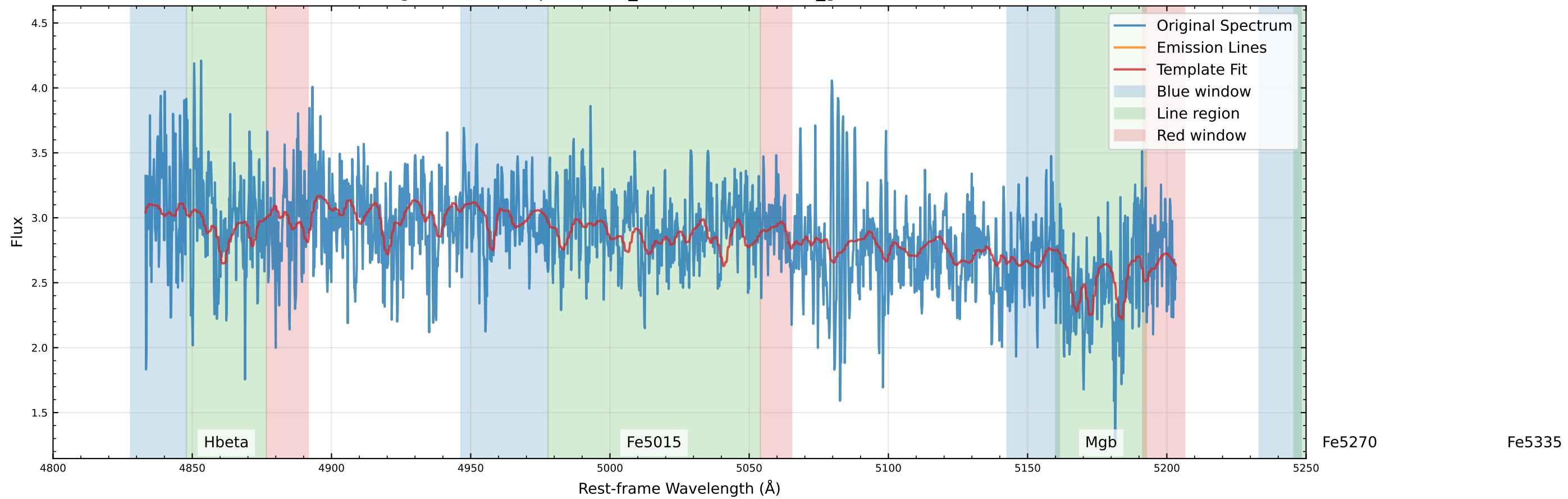
Original Data Comparison (v_star=-110.7 km/s, v_gas=-410.7 km/s)
