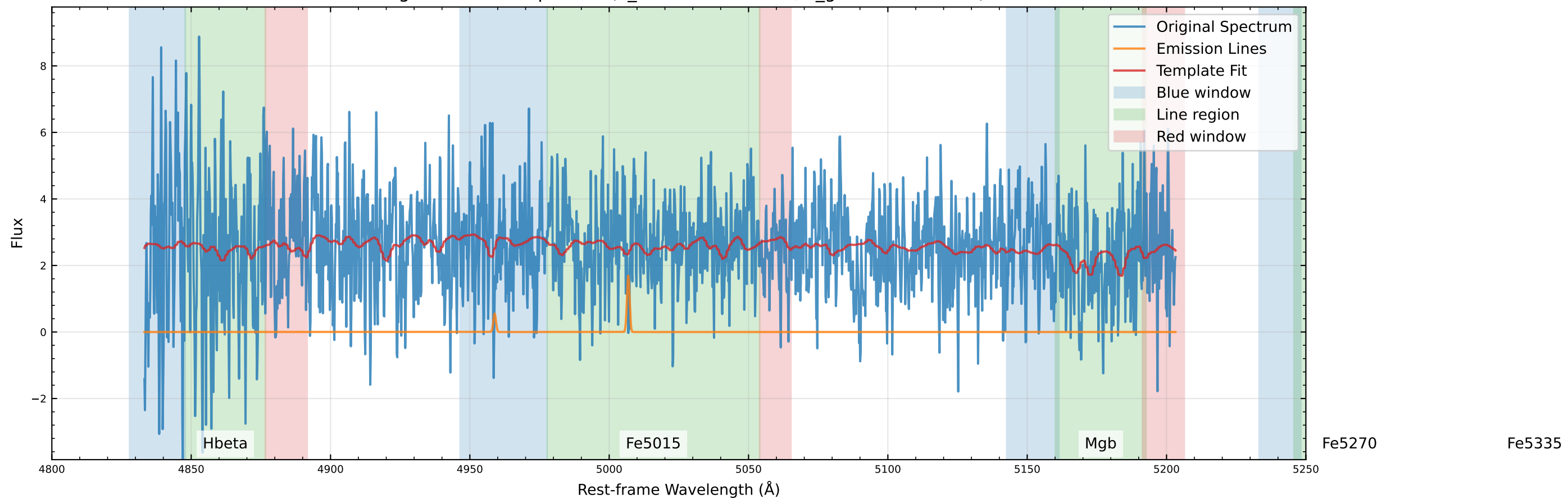
Original Data Comparison (v_star=-120.5 km/s, v_gas=-102.6 km/s)
