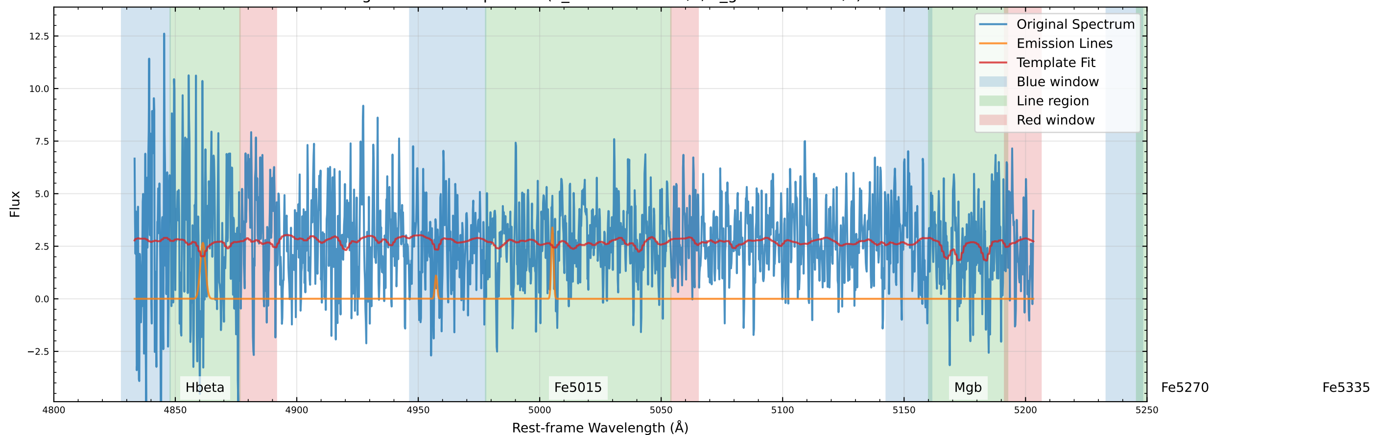
Original Data Comparison (v_star=142.4 km/s, v_gas=221.0 km/s)
