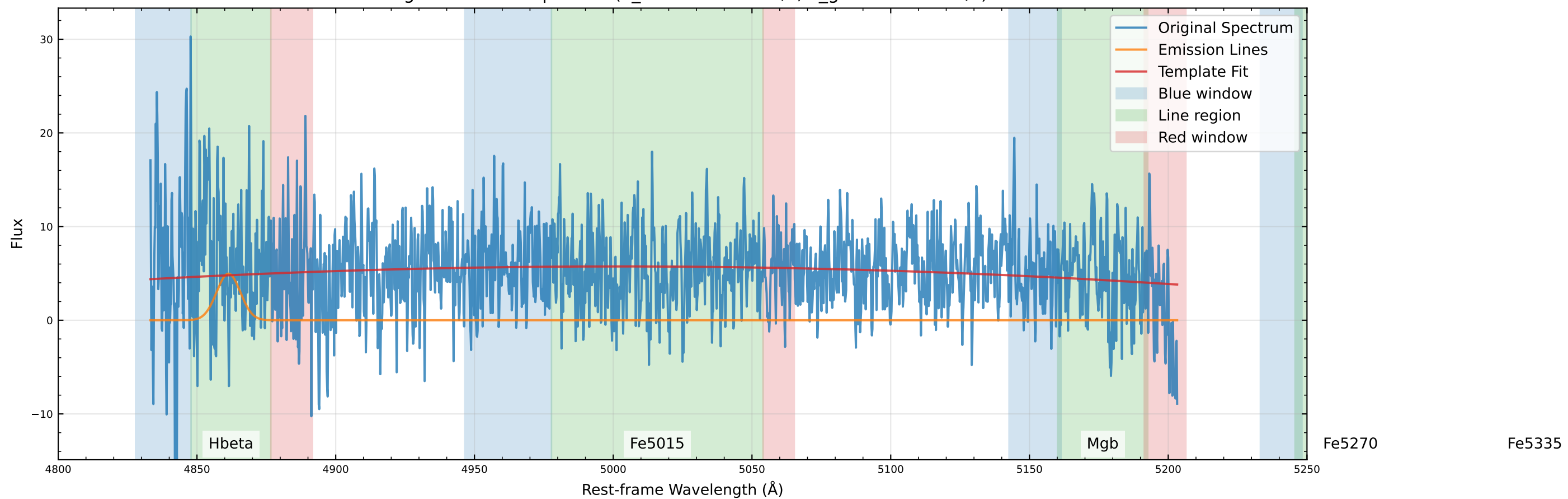
Original Data Comparison (v_star=-393.9 km/s, v_gas=-608.3 km/s)
