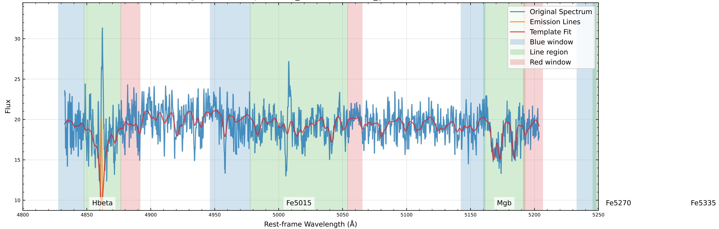
Original Data Comparison (v_star=30.1 km/s, v_gas=50.2 km/s)
