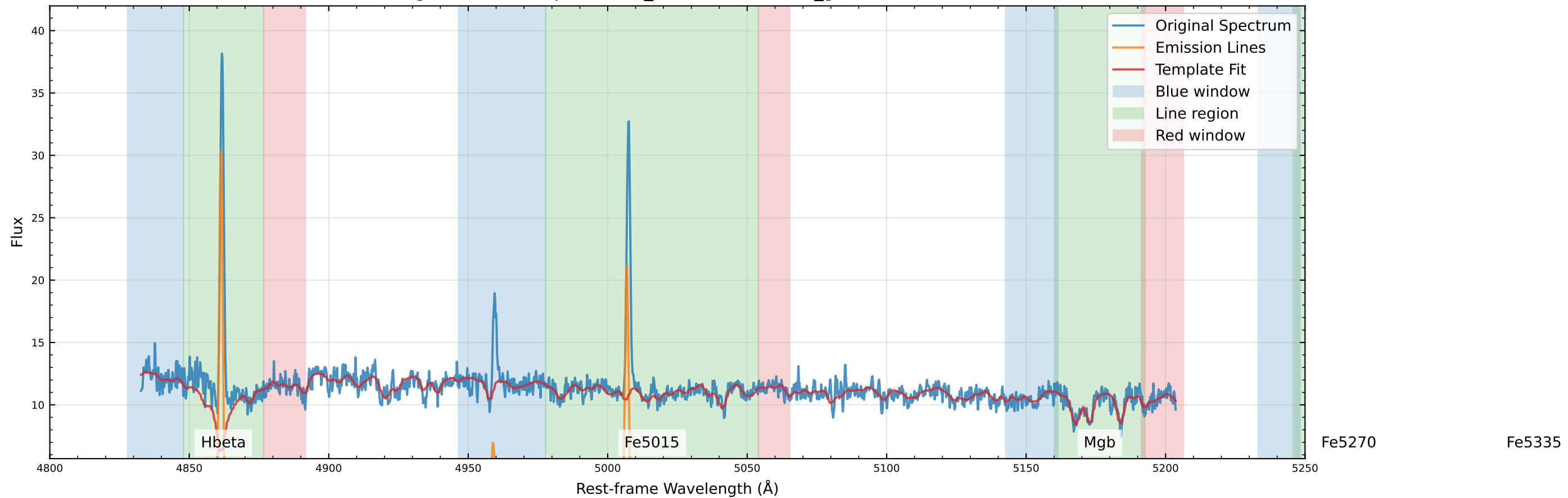
Original Data Comparison (v_star=10.1 km/s, v_gas=28.6 km/s)
