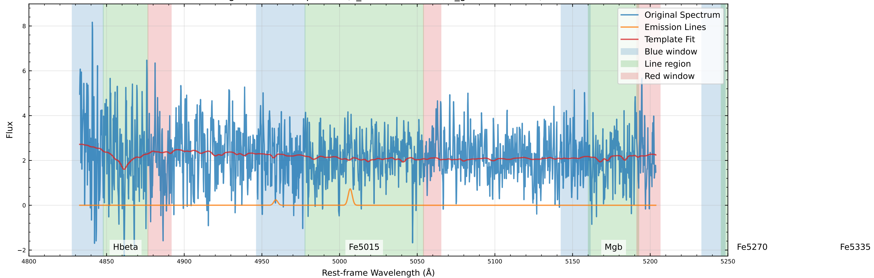
Original Data Comparison (v_star=-48.5 km/s, v_gas=-54.1 km/s)
