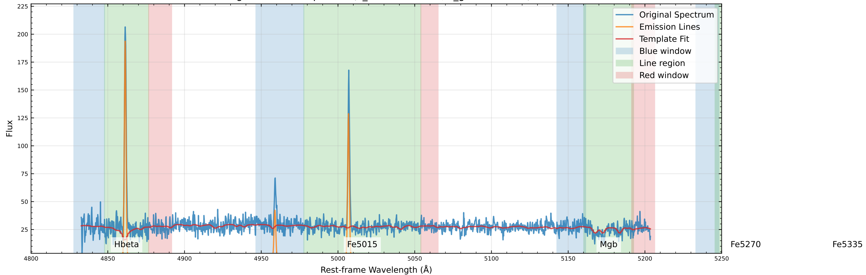
Original Data Comparison ( v_{\text{star}}=-1.9 km/s, v_{\text{gas}}=8.3 km/s)
