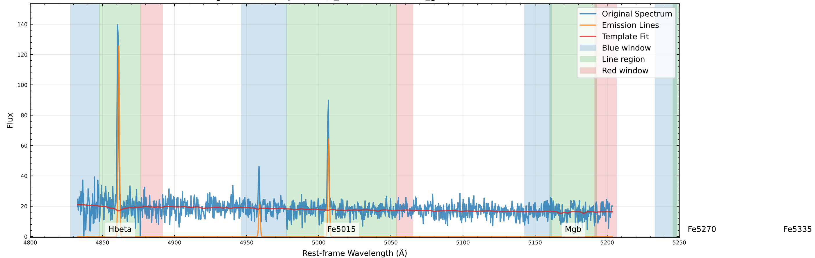
Original Data Comparison (v_star=-60.3 km/s, v_gas=-31.7 km/s)
