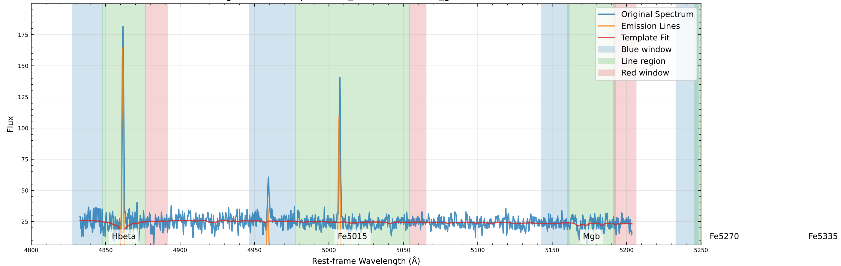
Original Data Comparison (v_star=31.6 km/s, v_gas=22.9 km/s)
