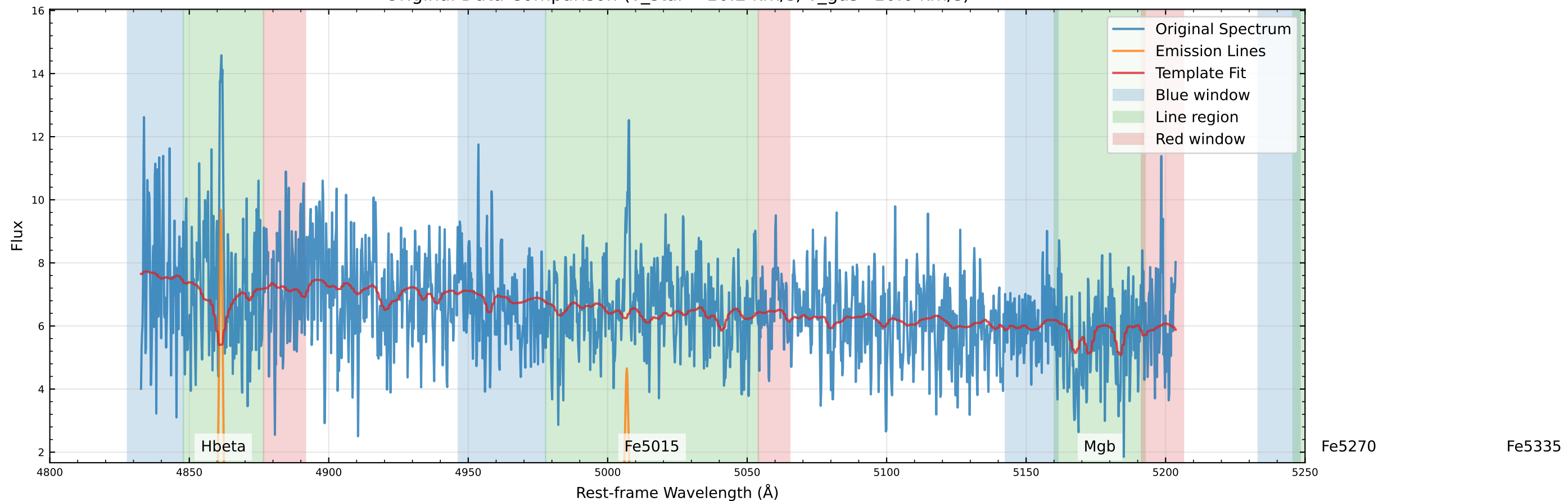
Original Data Comparison (v_star=-10.2 km/s, v_gas=10.6 km/s)
