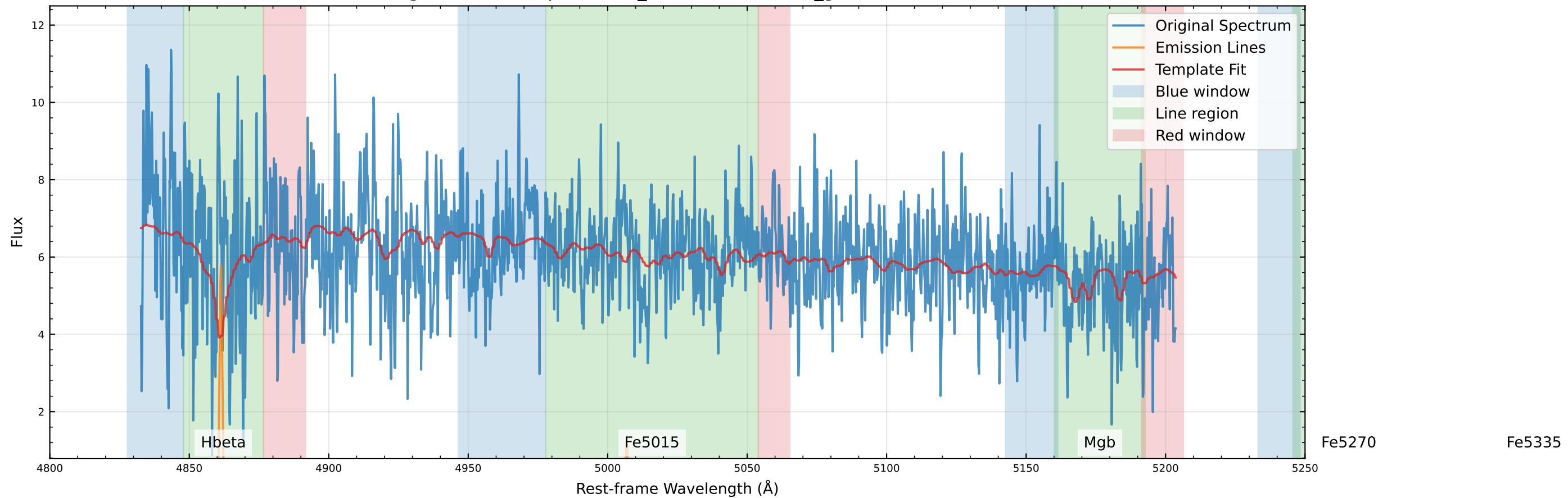
Original Data Comparison (v_star=-68.3 km/s, v_gas=-47.4 km/s)
