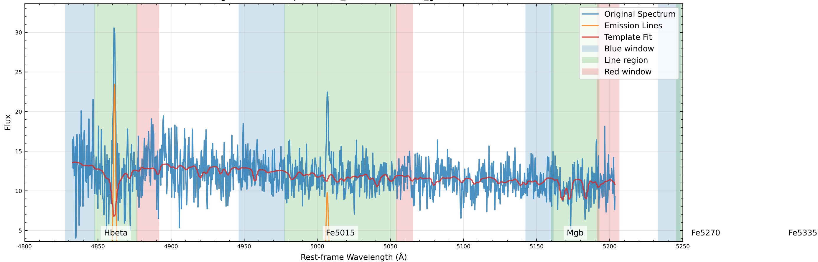
Original Data Comparison (v_star=0.0 km/s, v_gas=-4.2 km/s)
