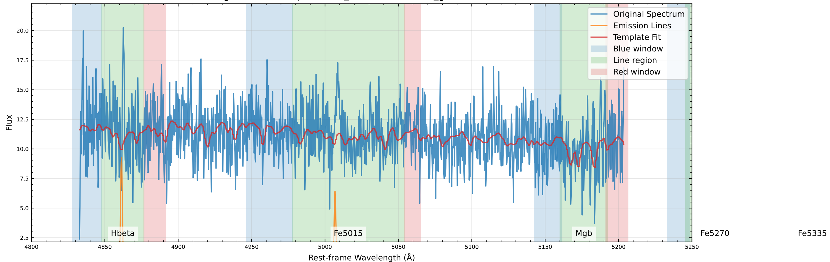
Original Data Comparison (v_star=41.9 km/s, v_gas=83.9 km/s)
