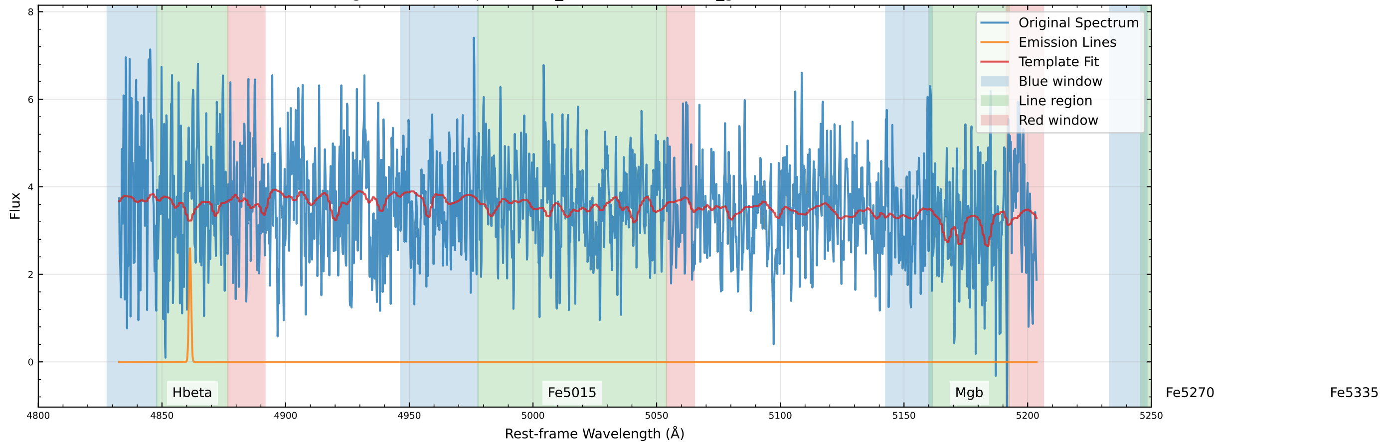
Original Data Comparison (v_star=197.3 km/s, v_gas=197.9 km/s)
