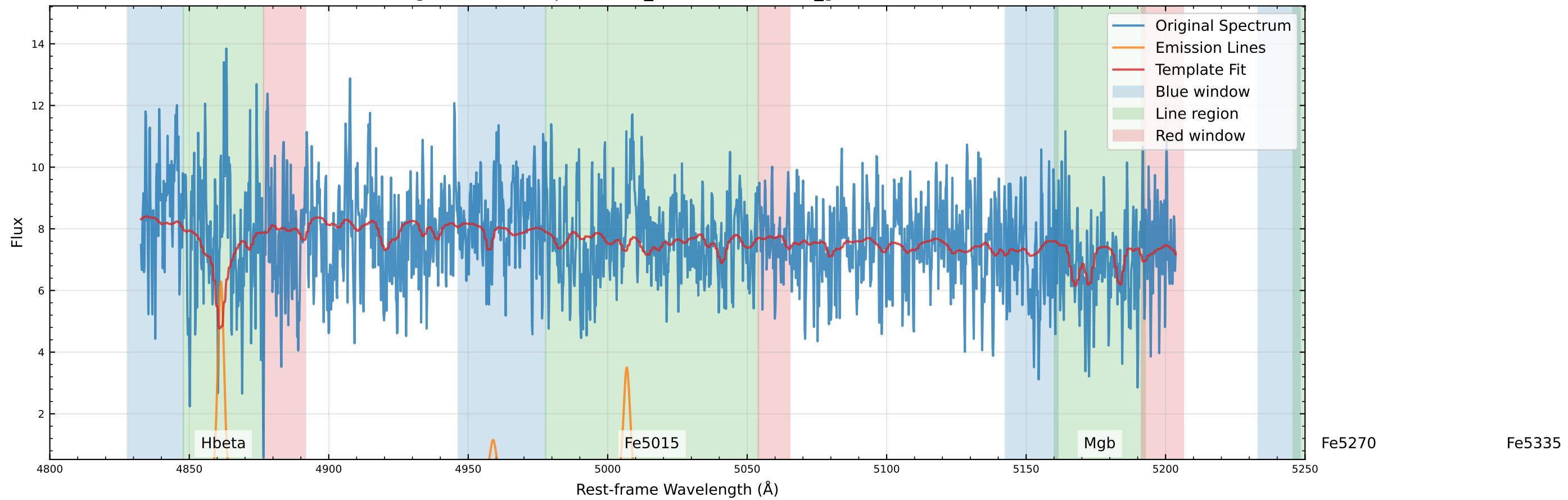
Original Data Comparison (v_star=14.8 km/s, v_gas=96.8 km/s)
