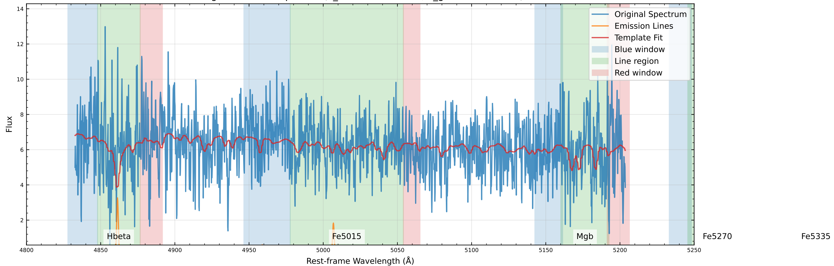
Original Data Comparison (v_star=-139.0 km/s, v_gas=-198.1 km/s)
