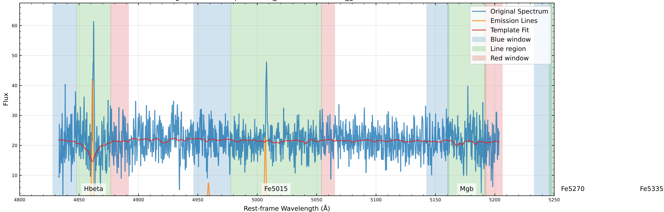
Original Data Comparison (v_star=64.9 km/s, v_gas=49.1 km/s)
