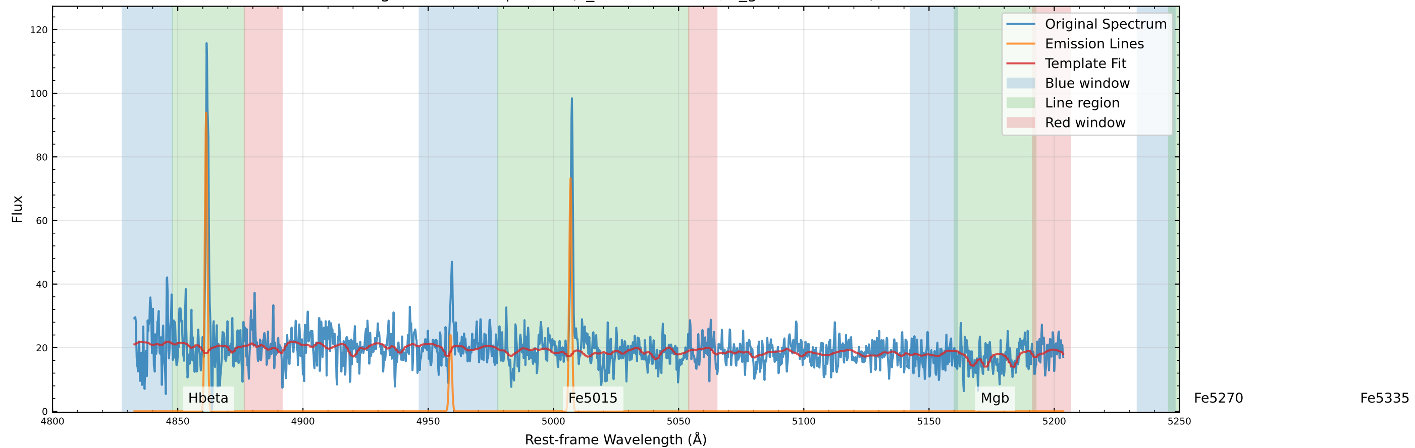
Original Data Comparison (v_star=38.2 km/s, v_gas=26.5 km/s)
