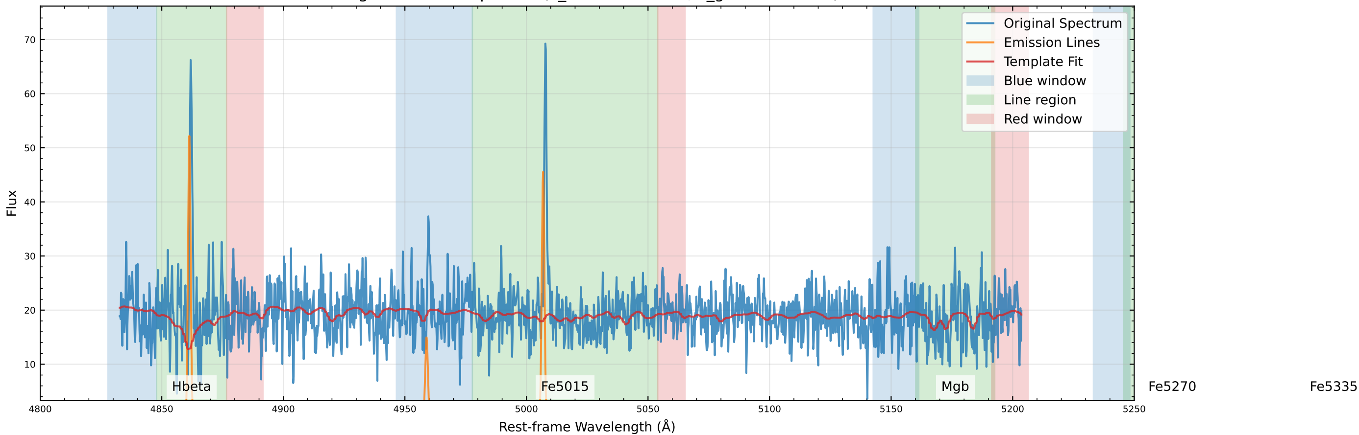
Original Data Comparison (v_star=30.2 km/s, v_gas=49.3 km/s)
