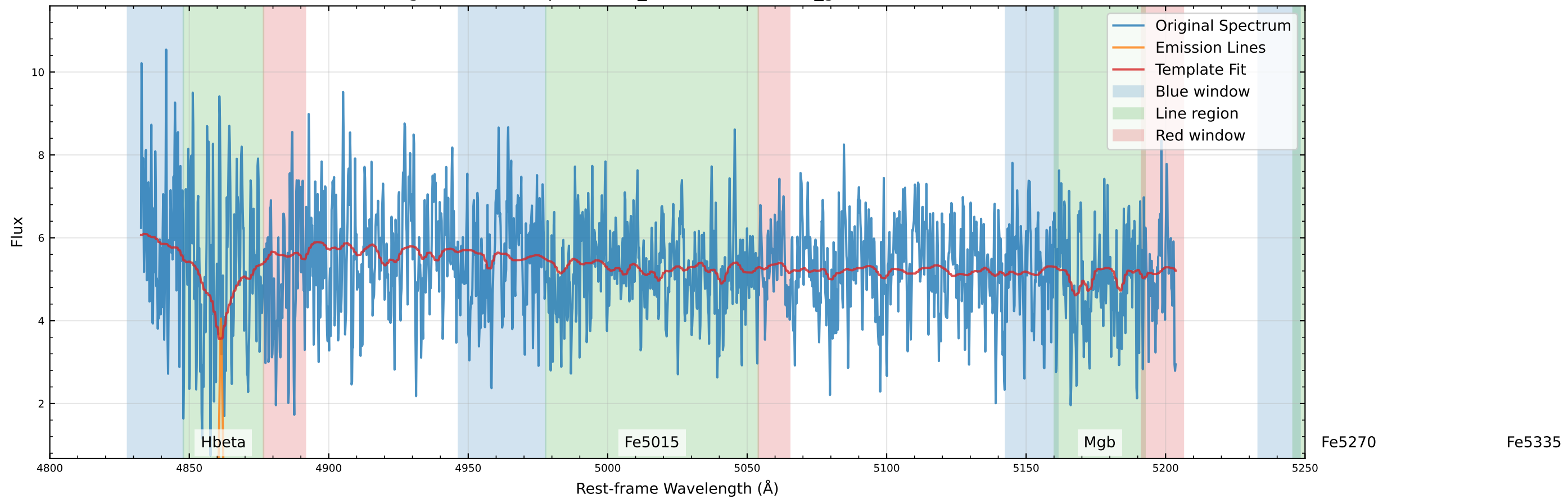
Original Data Comparison ( v_{\text{star}}=-28.4 km/s, v_{\text{gas}}=-29.0 km/s)
