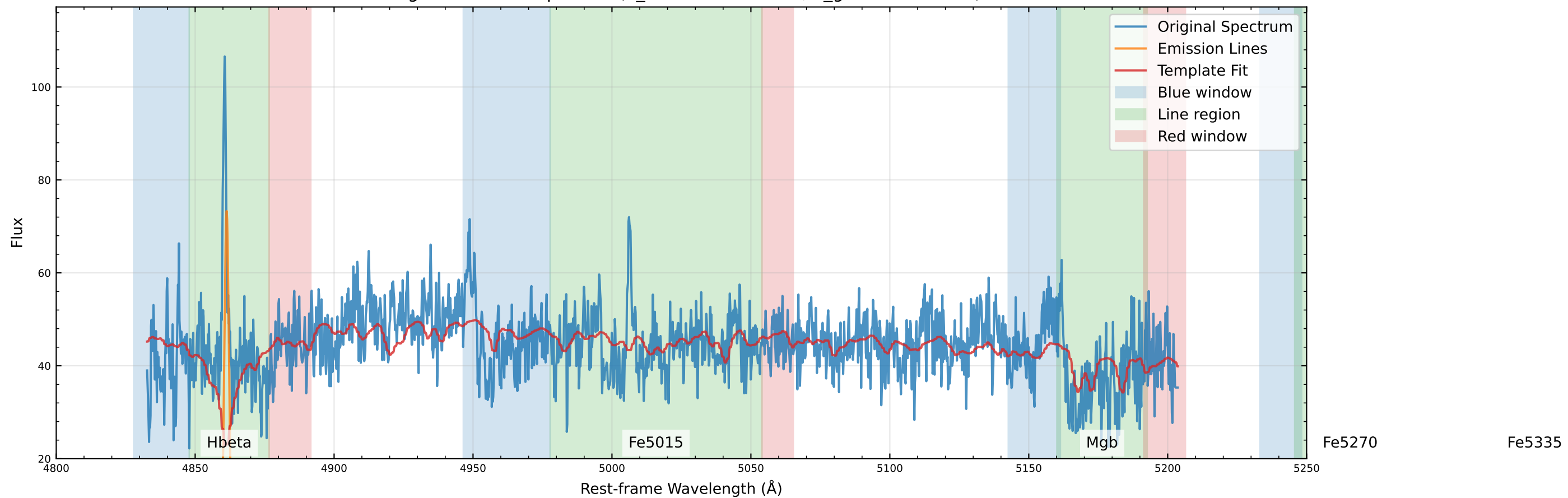
Original Data Comparison (v_star=-109.3 km/s, v_gas=-48.8 km/s)
