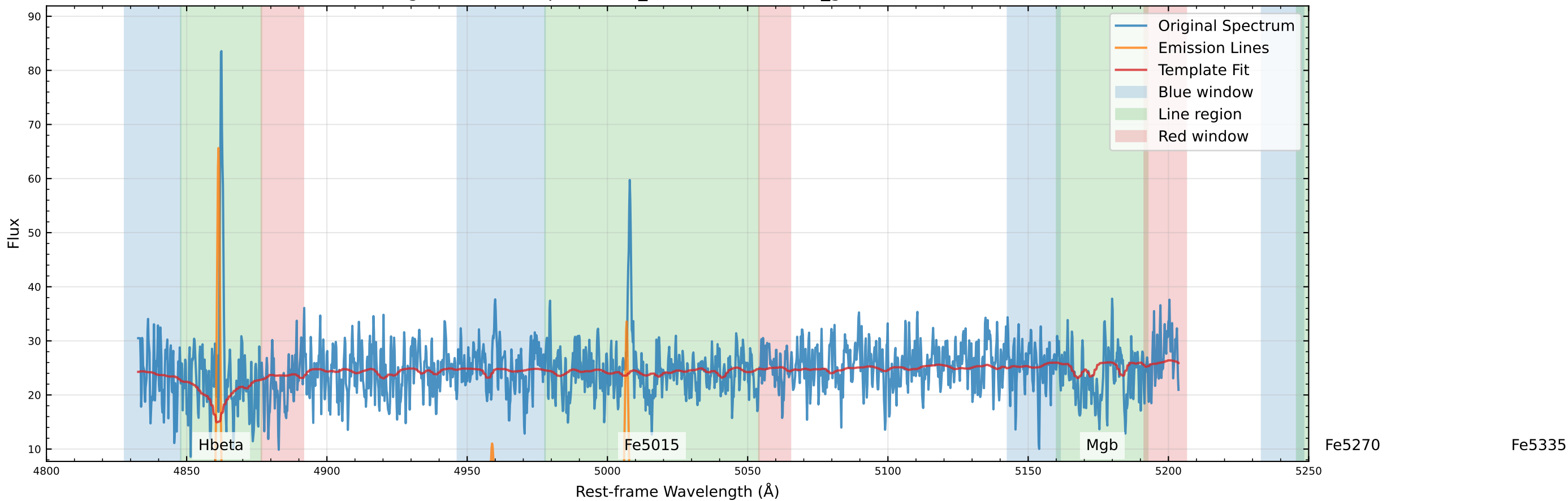
Original Data Comparison (v_star=104.3 km/s, v_gas=66.8 km/s)
