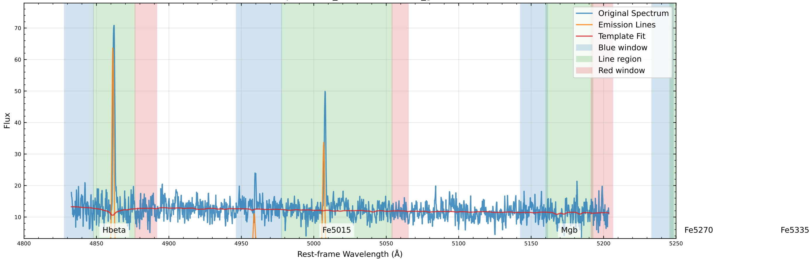
Original Data Comparison (v_star=45.0 km/s, v_gas=45.1 km/s)
