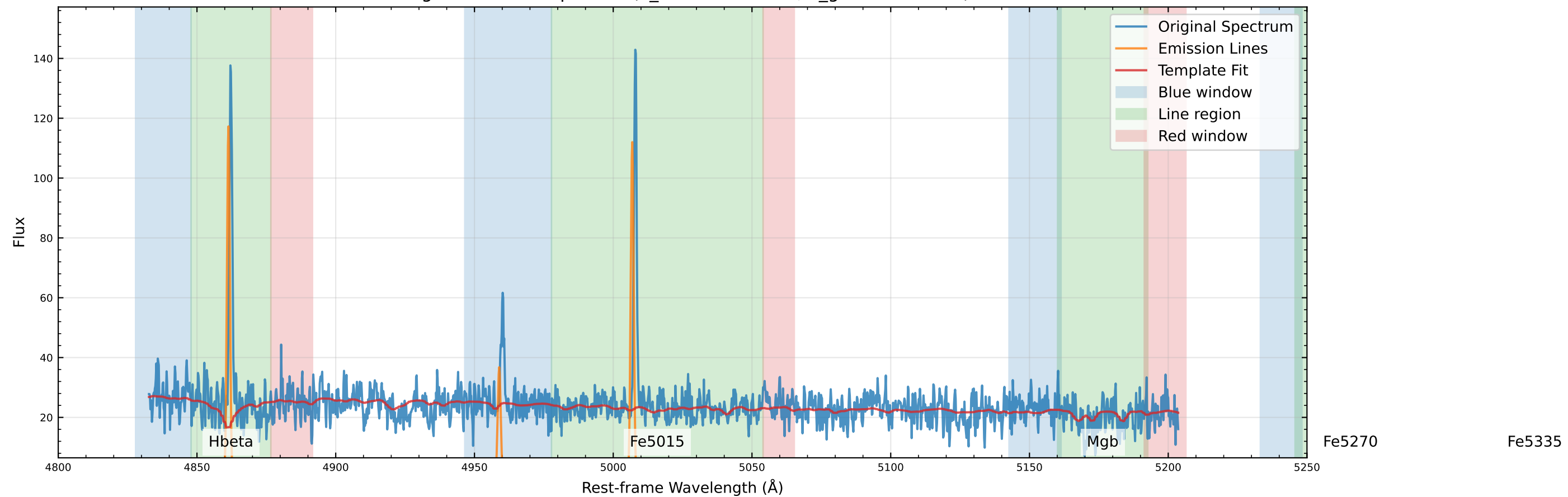
Original Data Comparison (v_star=41.8 km/s, v_gas=60.6 km/s)
