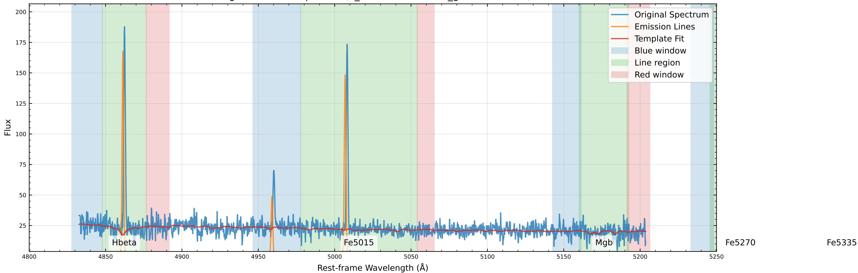
Original Data Comparison (v_star=69.8 km/s, v_gas=71.6 km/s)
