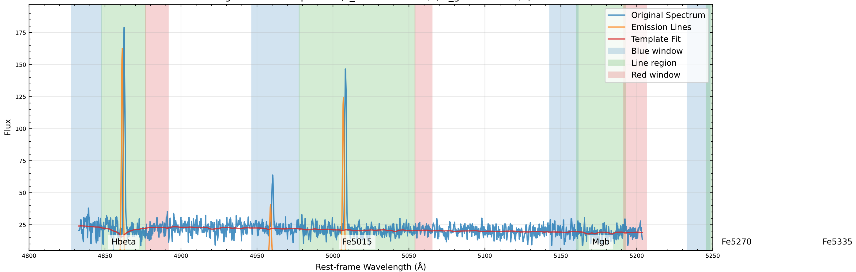
Original Data Comparison (v_star=103.2 km/s, v_gas=79.5 km/s)
