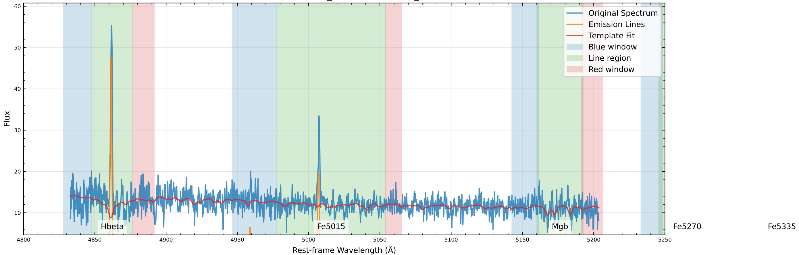
Original Data Comparison (v_star=21.8 km/s, v_gas=22.7 km/s)
