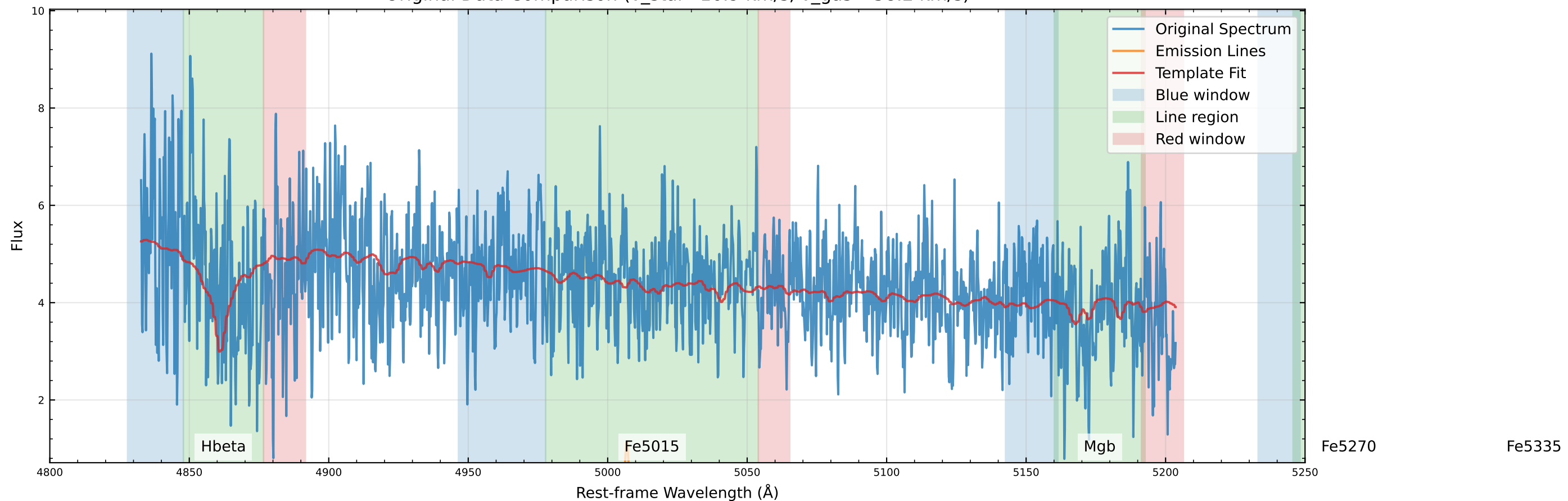
Original Data Comparison (v_star=16.9 km/s, v_gas=-58.2 km/s)
