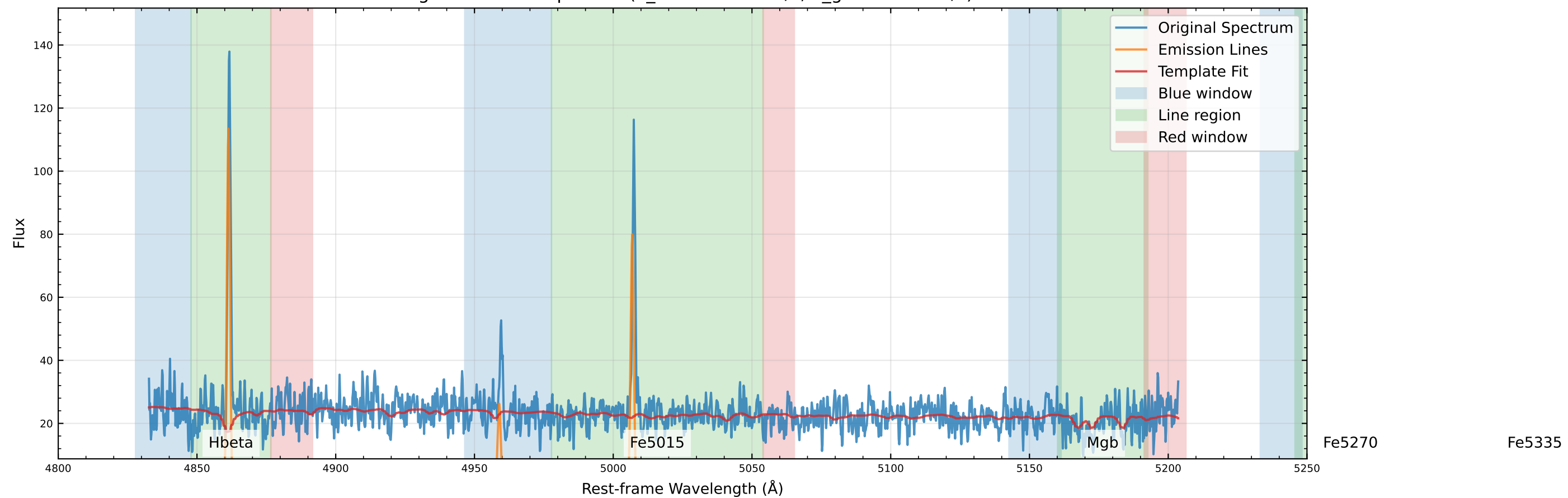
Original Data Comparison (v_star=-15.9 km/s, v_gas=24.8 km/s)
