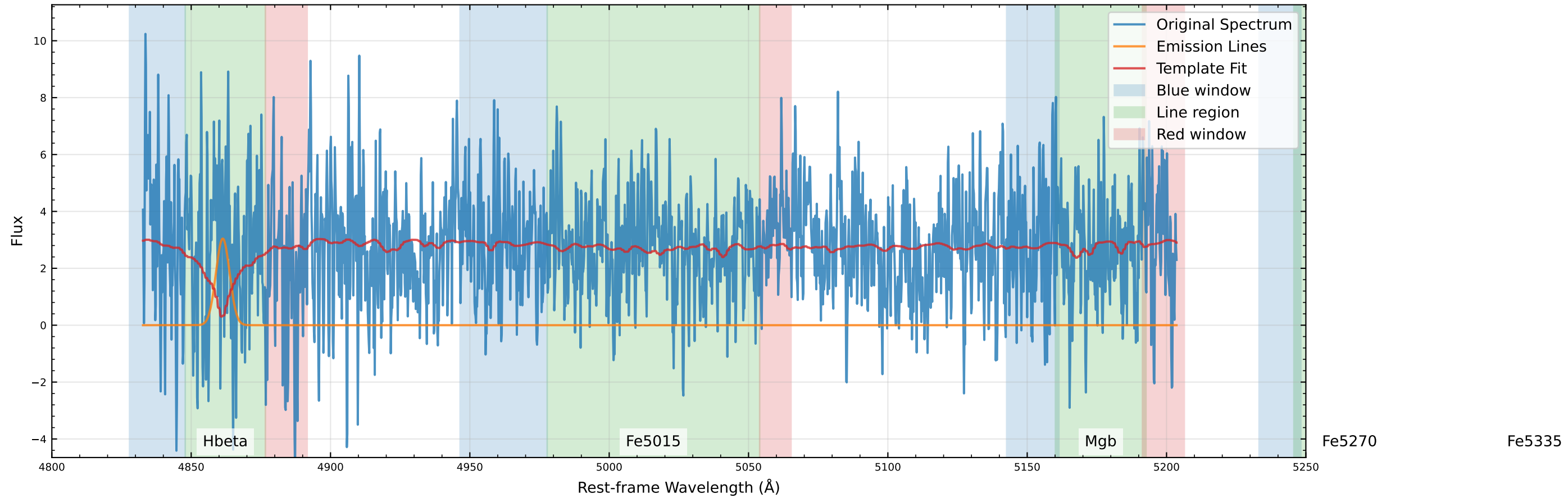
Original Data Comparison (v_star=-44.7 km/s, v_gas=-72.2 km/s)
