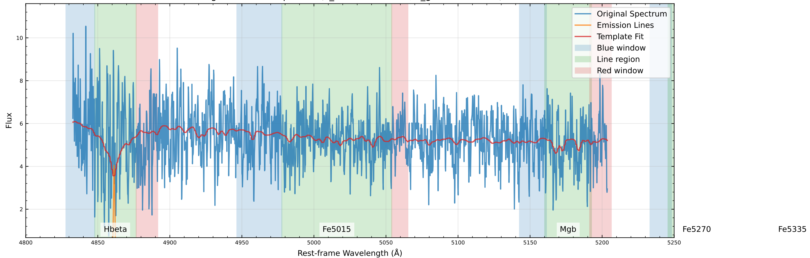
Original Data Comparison (v_star=-28.4 km/s, v_gas=-29.0 km/s)
