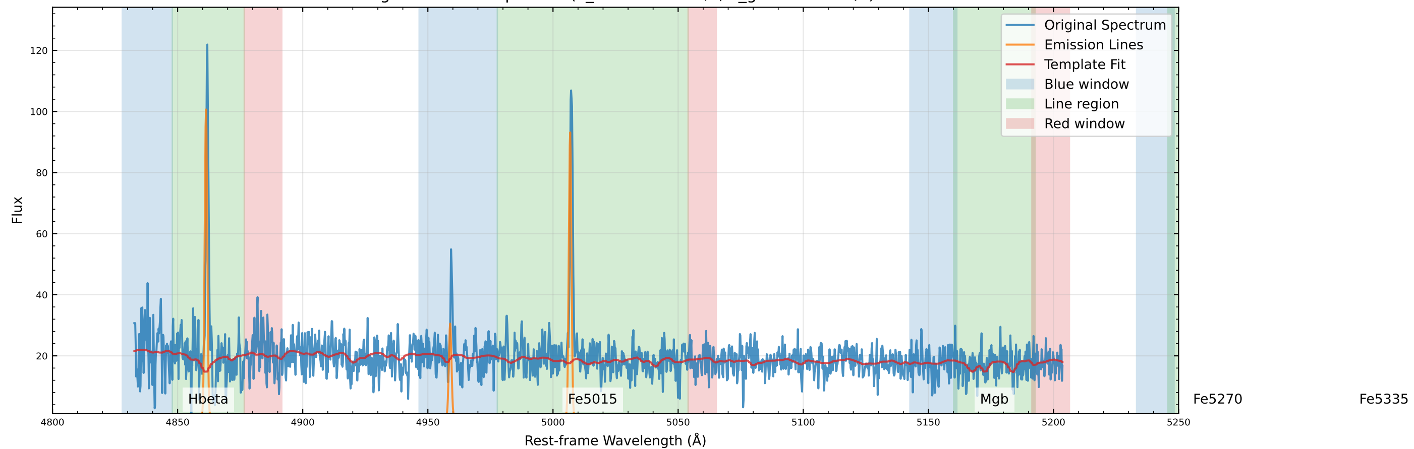
Original Data Comparison (v_star=49.1 km/s, v_gas=29.9 km/s)
